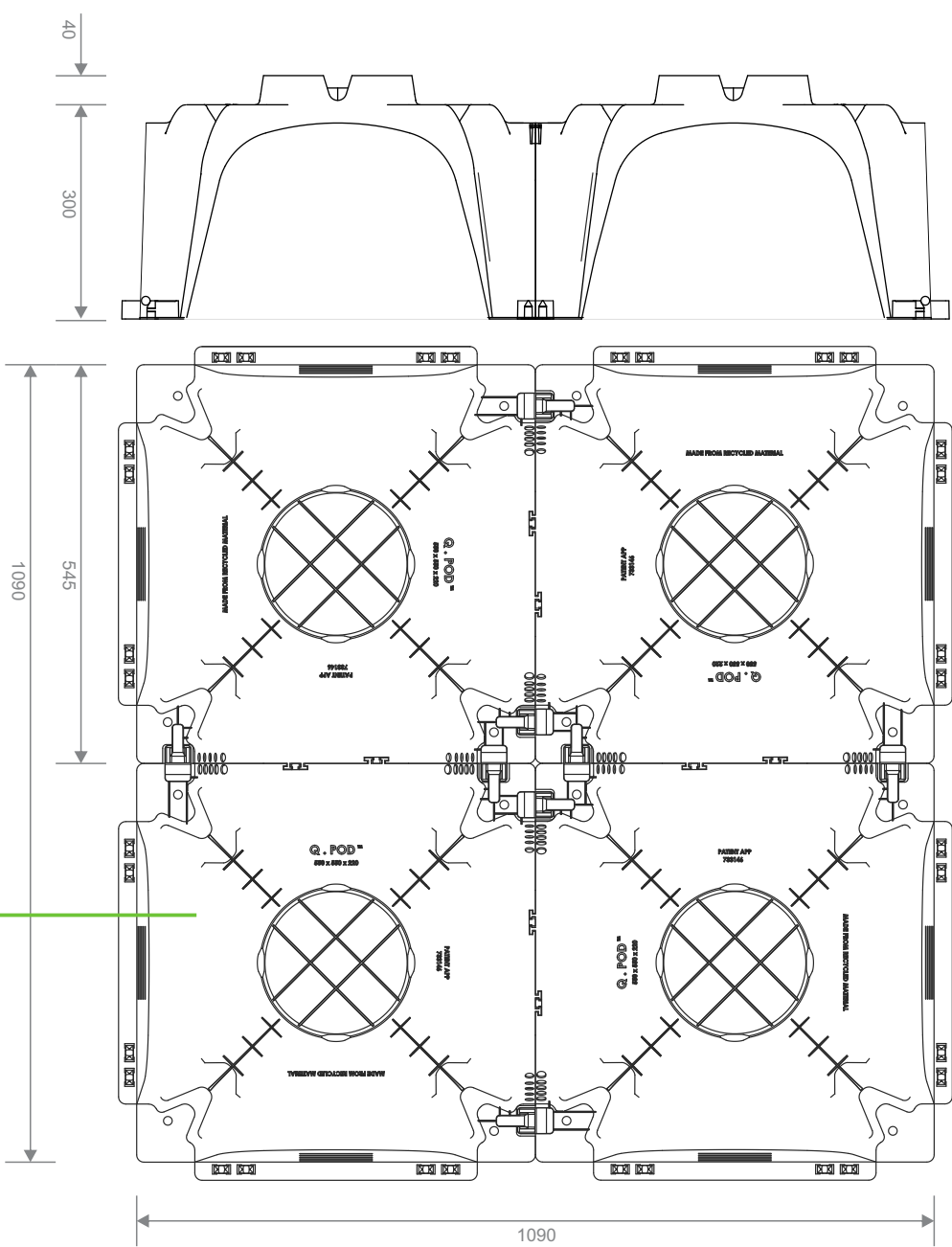
4x QPOD™ Closed Side Volume: 0.331m3
