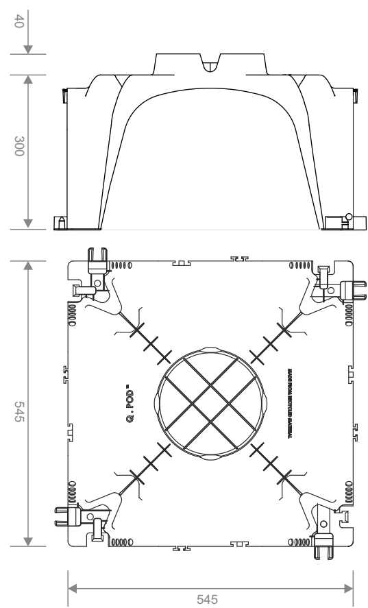
Individual QPOD™ 300 Closed 2 Side Volume: 0.0828m3
